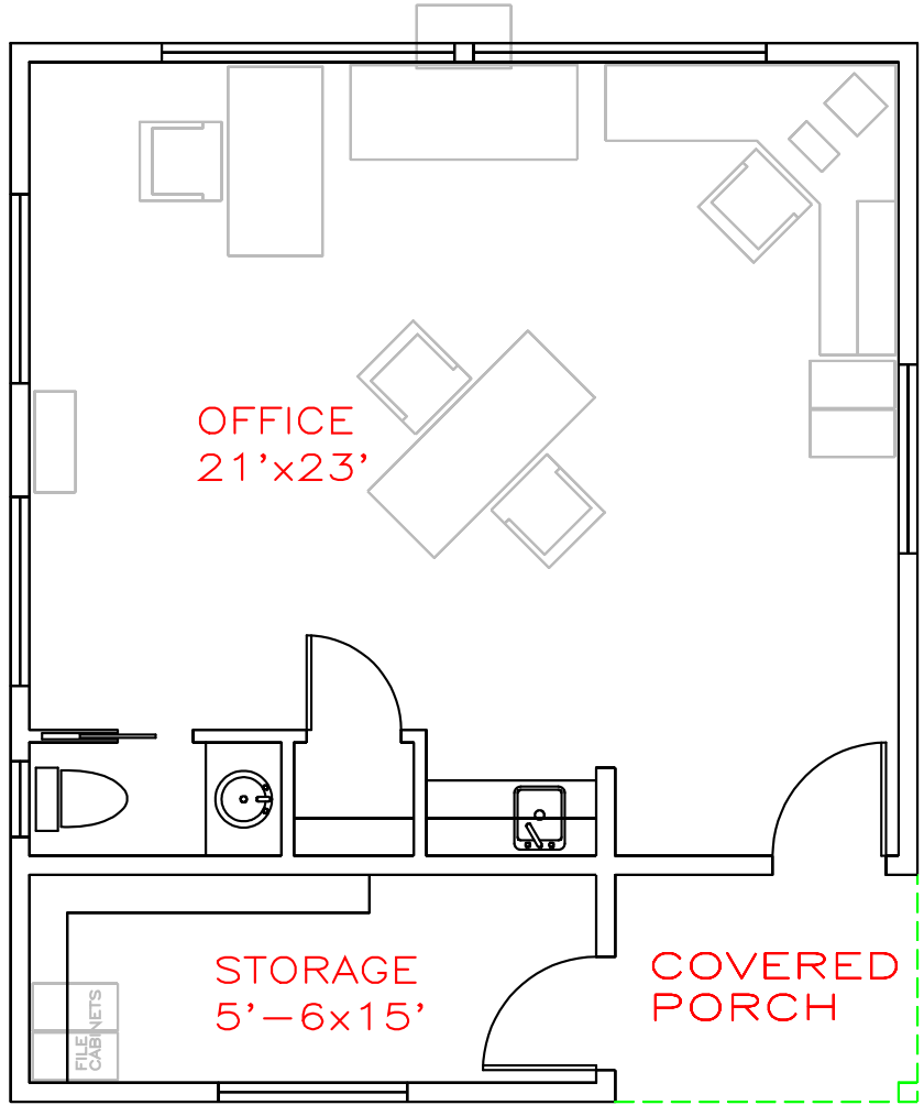
MAIN FLOOR PLAN VIEW
