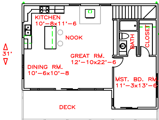
UPPER FLOOR PLAN VIEW
