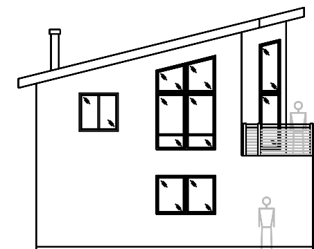
LEFT SIDE ELEV. VIEW
