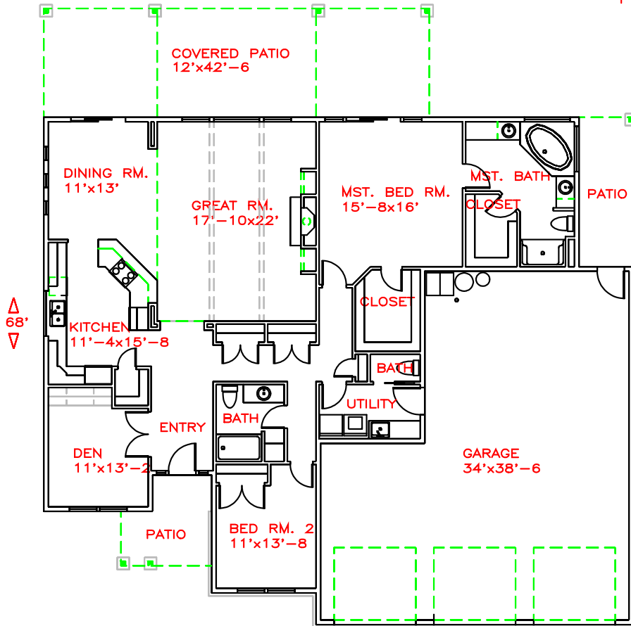
MAIN FLOOR PLAN VIEW
