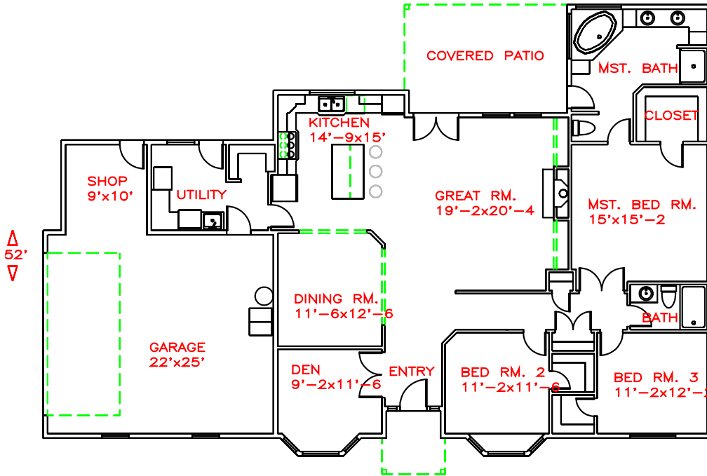
MAIN FLOOR PLAN VIEW
