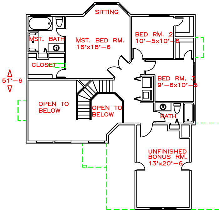
UPPER FLOOR PLAN VIEW
