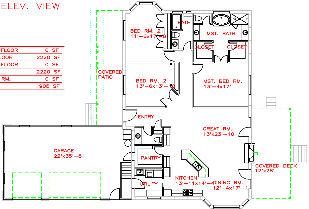
MAIN FLOOR PLAN VIEW
