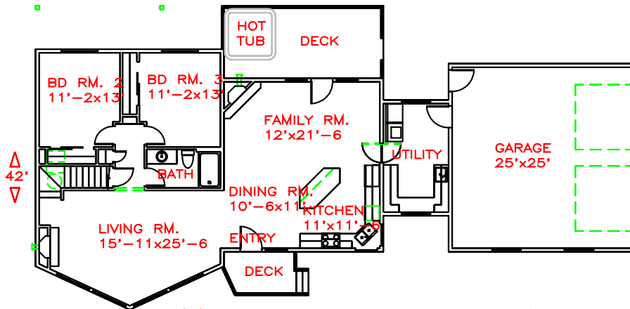
MAIN FLOOR PLAN VIEW
