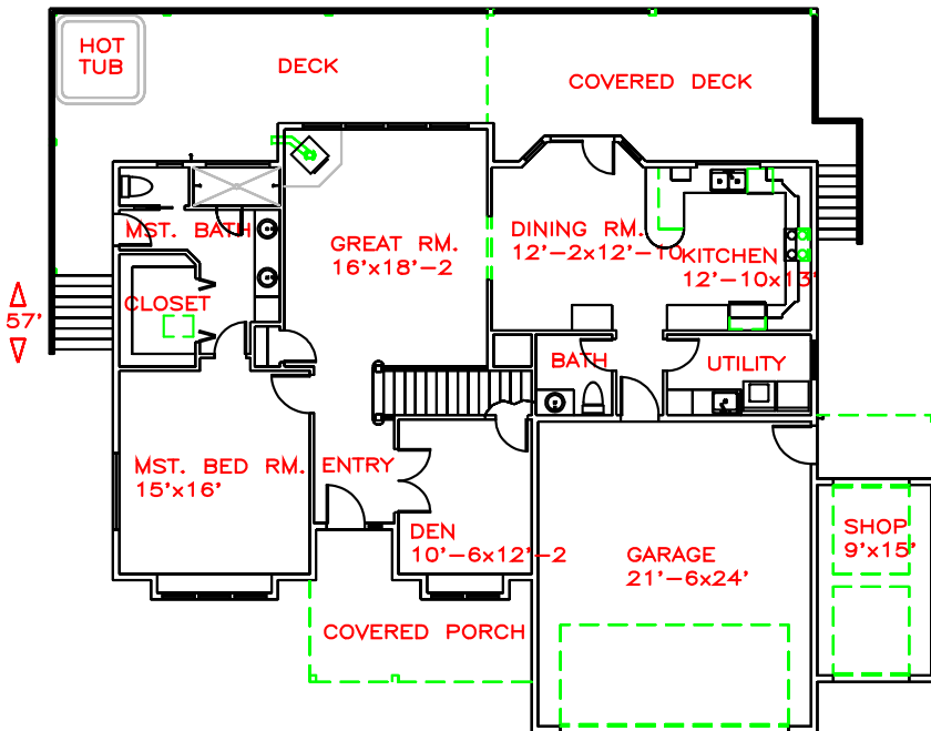
MAIN FLOOR PLAN VIEW
