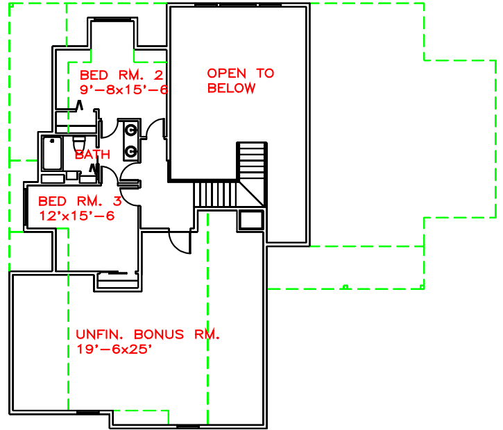
UPPER FLOOR PLAN VIEW
