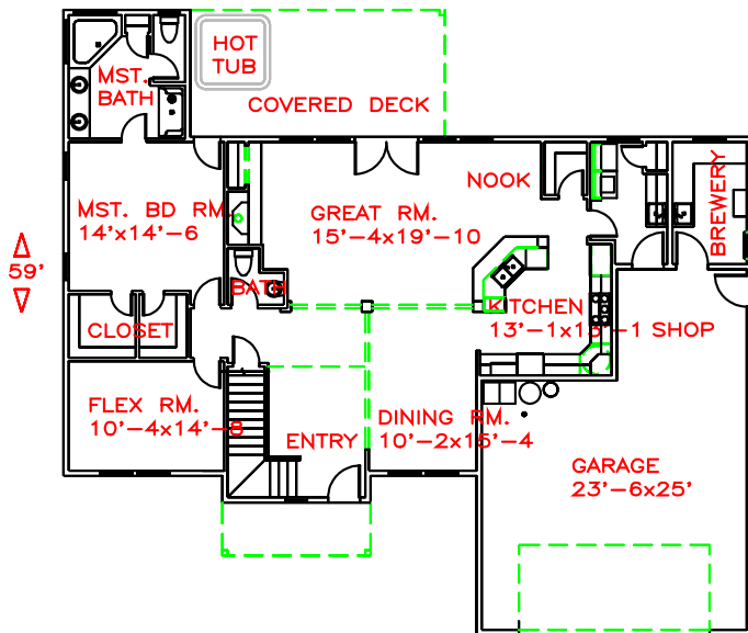
MAIN FLOOR PLAN VIEW
