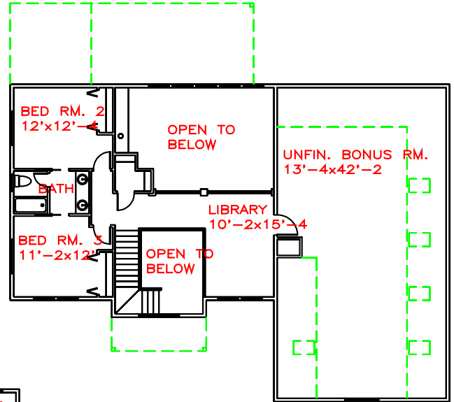
UPPER FLOOR PLAN VIEW
