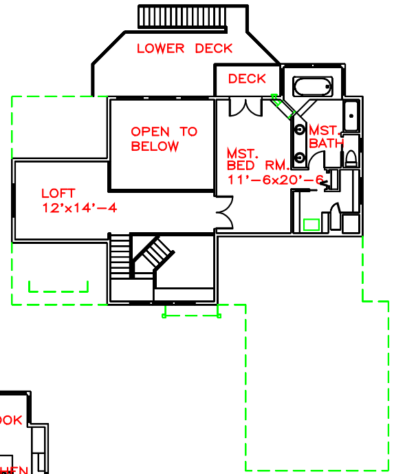
UPPER FLOOR PLAN VIEW
