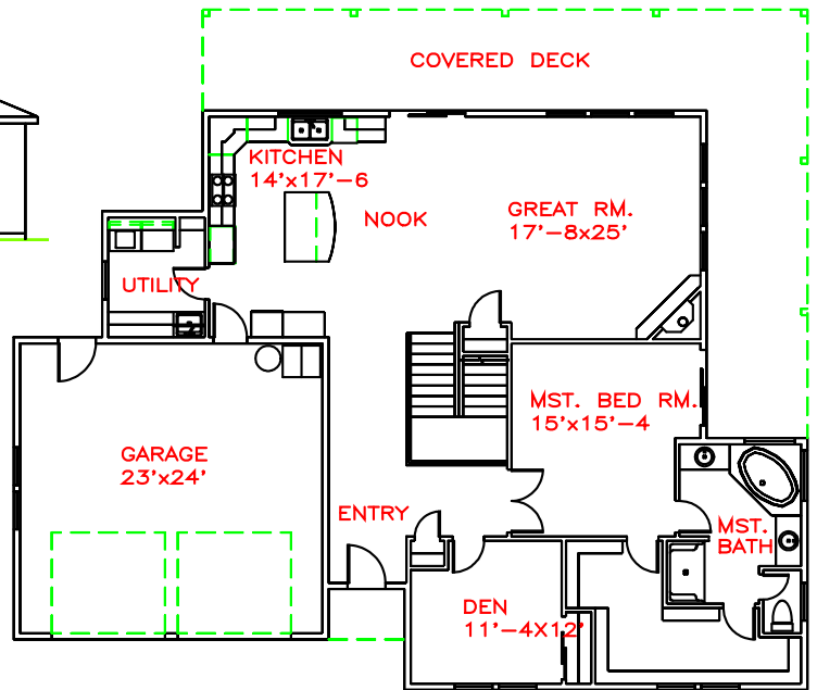
UPPER FLOOR PLAN VIEW < 63' >
