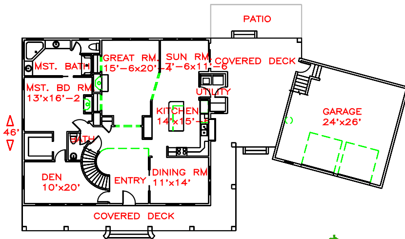
MAIN FLOOR PLAN VIEW
