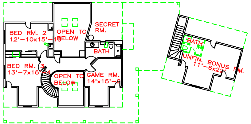
UPPER FLOOR PLAN VIEW
