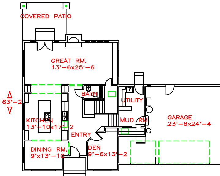
MAIN FLOOR PLAN VIEW
