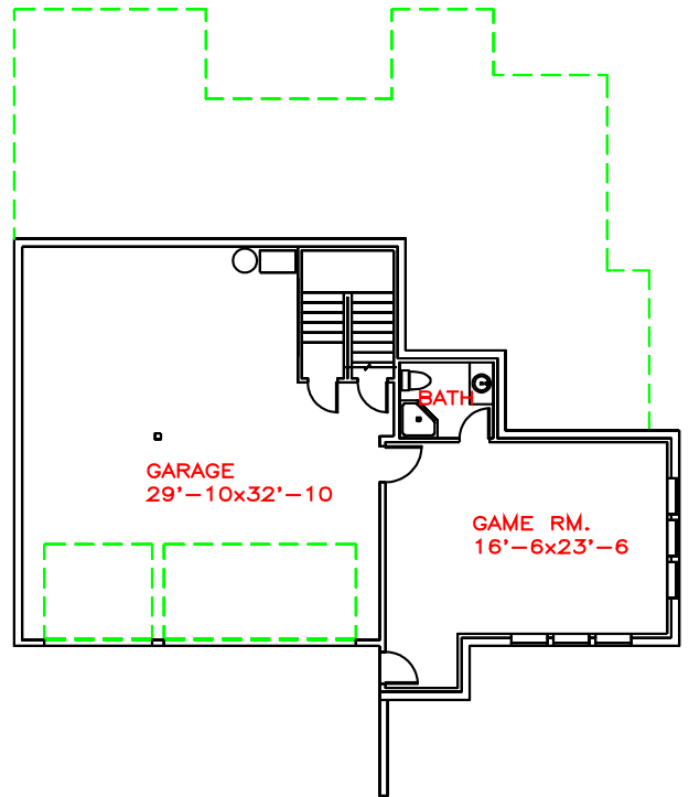
LOWER FLOOR PLAN VIEW
