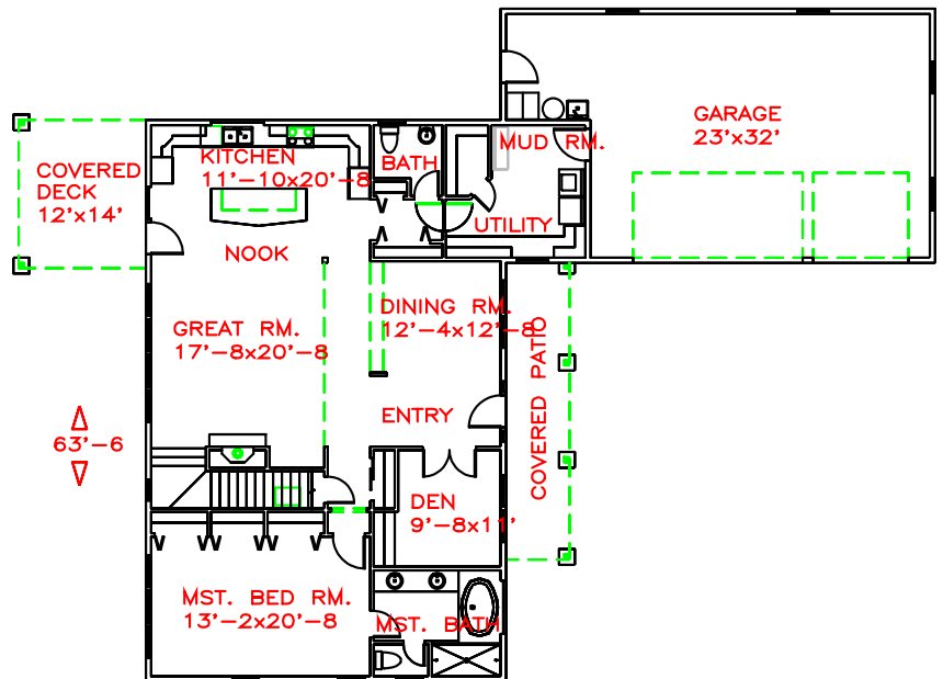
MAIN FLOOR PLAN VIEW
