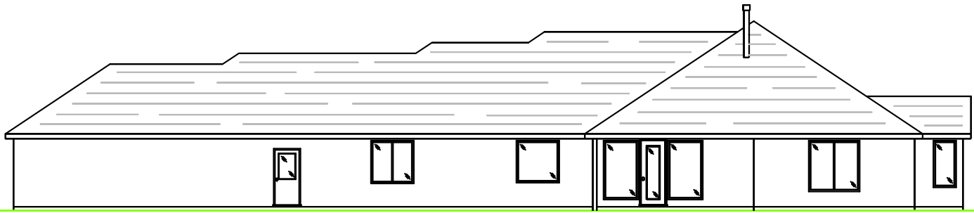
REAR ELEV. VIEW
