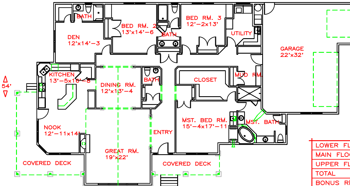
MAIN FLOOR PLAN VIEW
