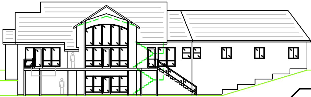
REAR ELEV. VIEW
