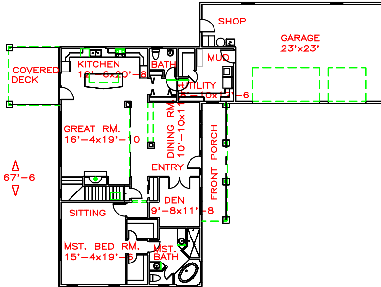
MAIN FLOOR PLAN VIEW
