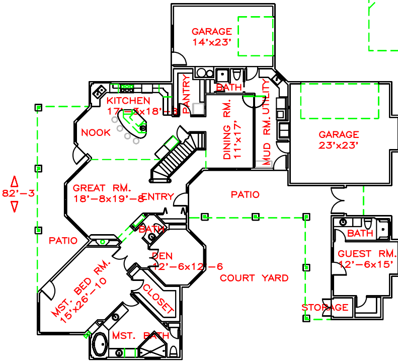
MAIN FLOOR PLAN VIEW
