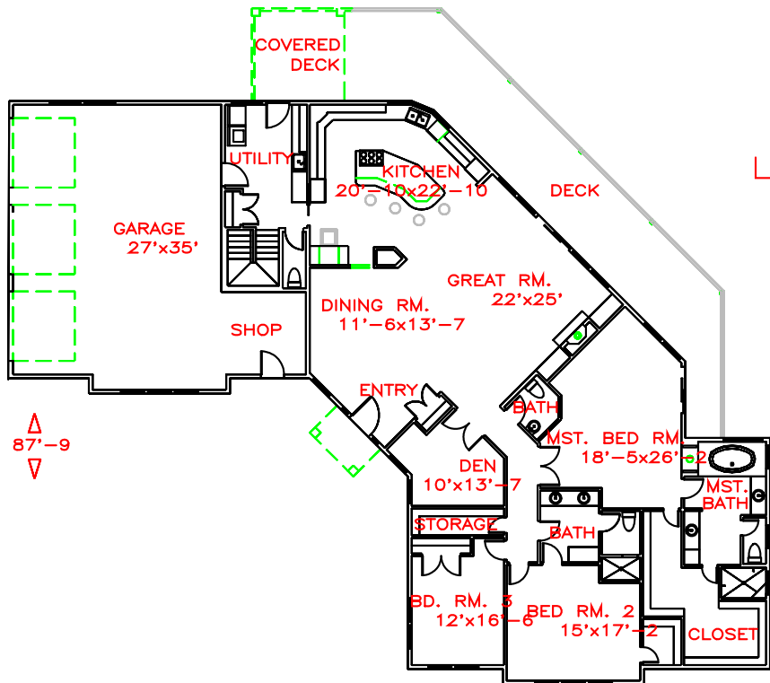
MAIN FLOOR PLAN VIEW
