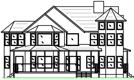
RIGHT SIDE ELEV. VIEW
