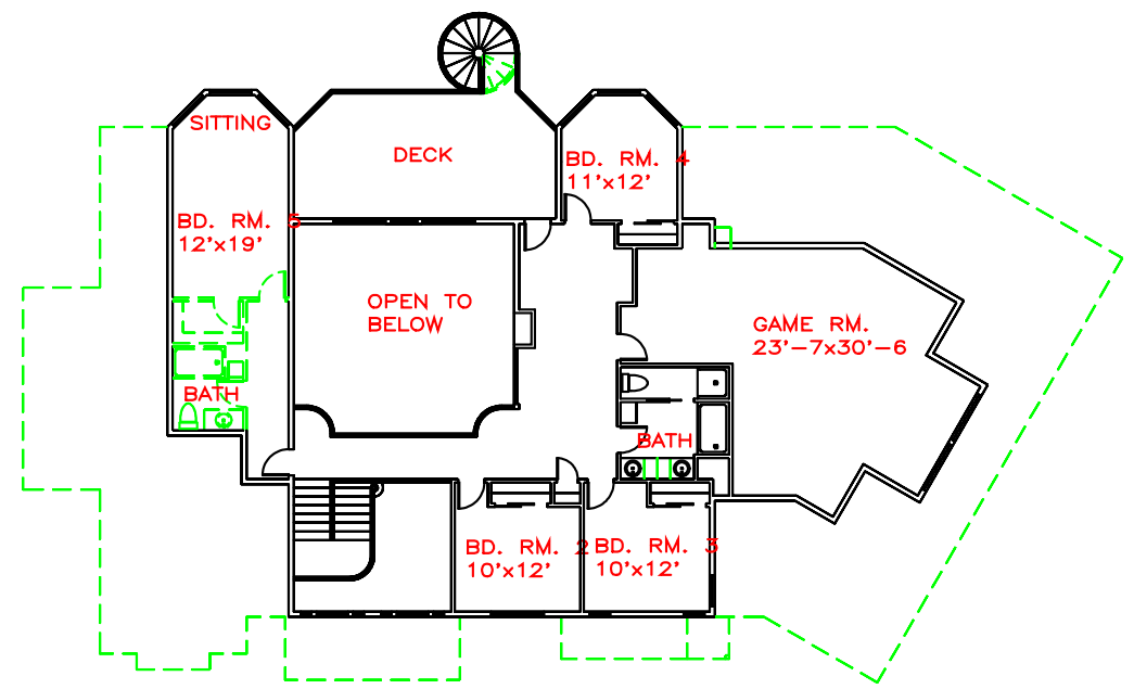
UPPER FLOOR PLAN VIEW
