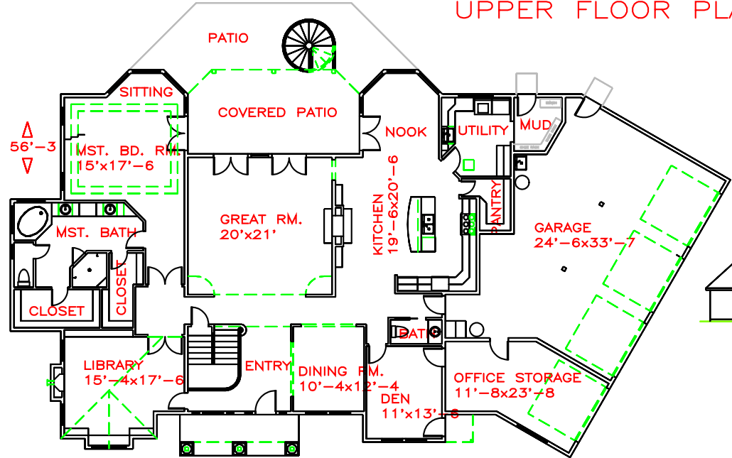
MAIN FLOOR PLAN VIEW
