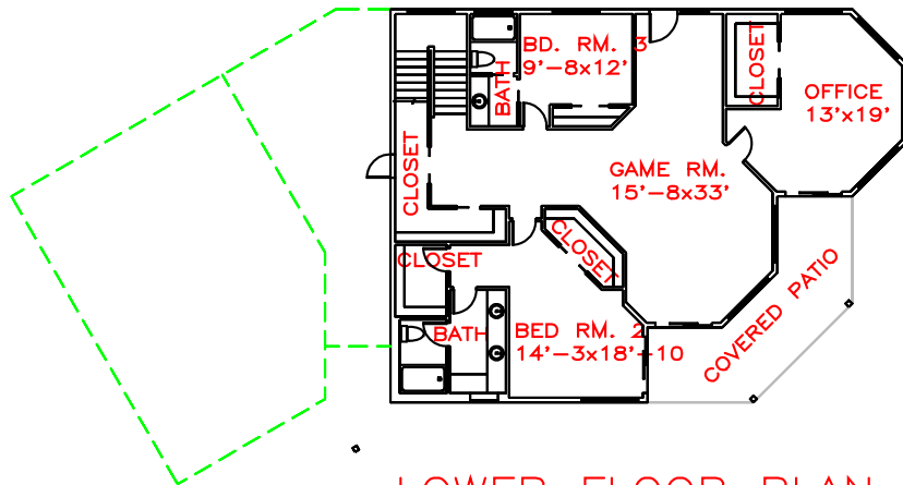
LOWER FLOOR PLAN VIEW
