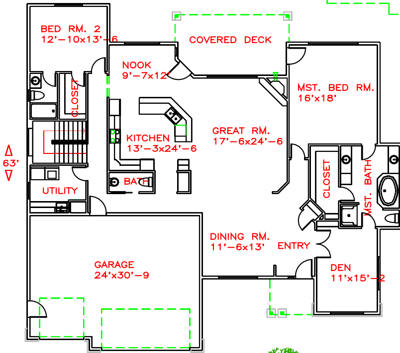
MAIN FLOOR PLAN VIEW ◀ 68' ▶
