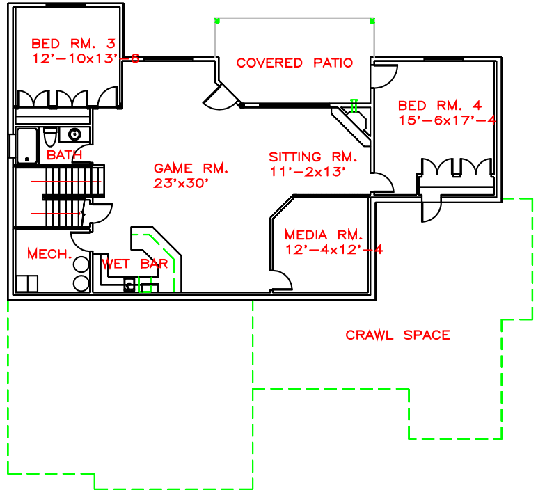
UPPER FLOOR PLAN VIEW
