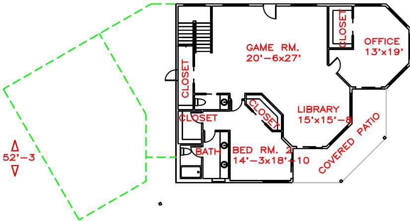
LOWER FLOOR PLAN VIEW
